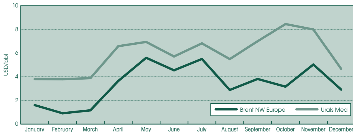
Graph 3: Refining Margins 2004
