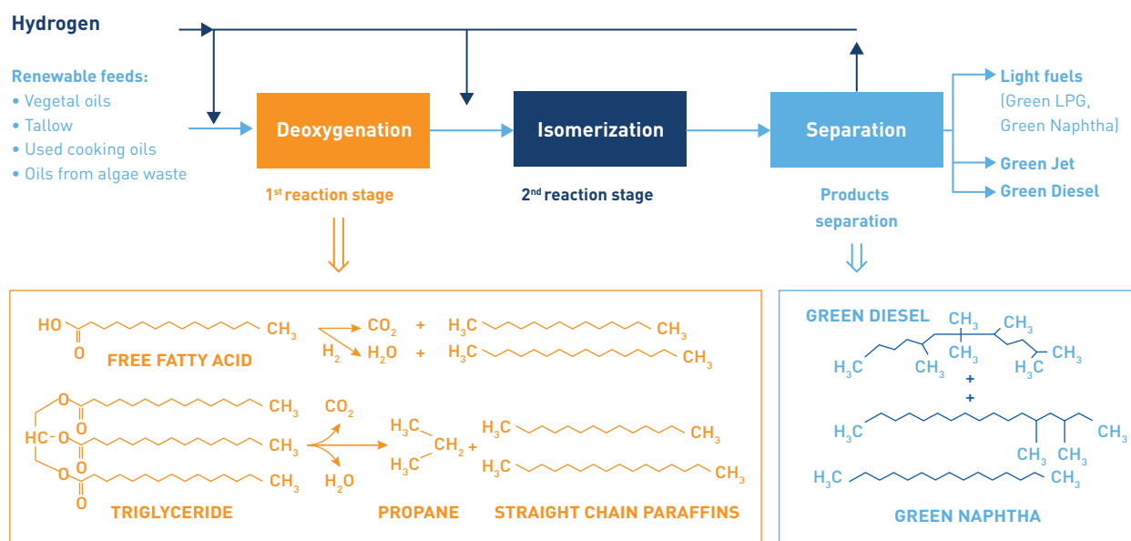
FIGURE 20: HYDROTREATED VEGETABLE OIL PRODUCTION PROCESS
